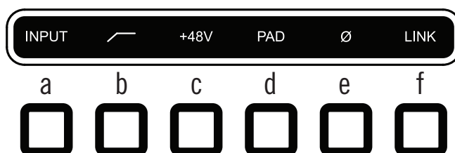
Apollo Twin's preamp option buttons
