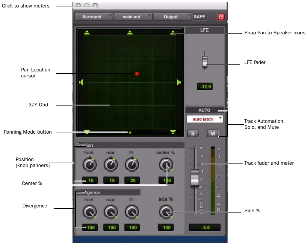
Figure 6. Output window with a 7.1 format multichannel panner
